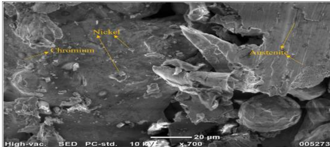
Figure 3 SEM image of LPBF SS 316L
